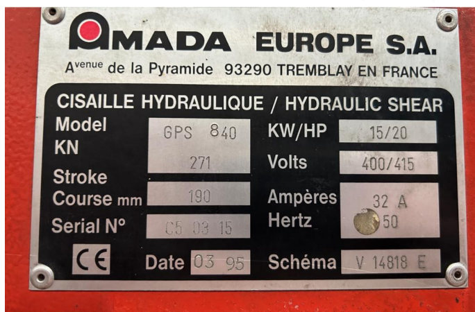
CISAILLE GUILLOTINE AMADA GPS 840 (3).webp
