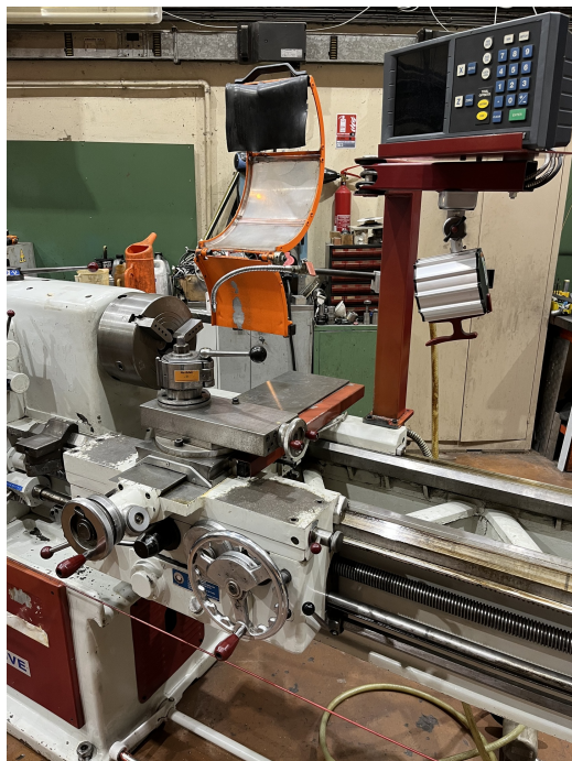
TOUR HORIZONTAL CAZENEUVE TYPE HB 575
